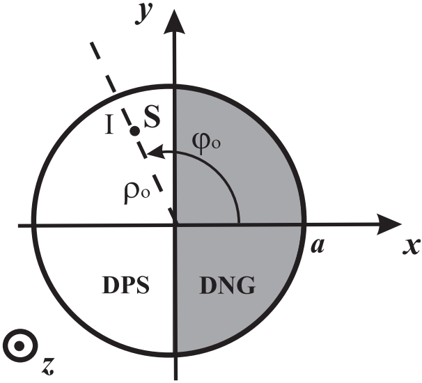
Fig. 1. Cross section of the resonator
