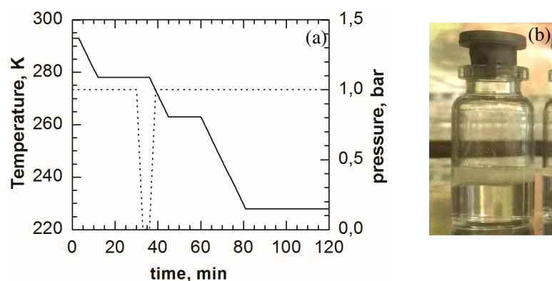
Fig. 1.(a) Evolution of pressure (--) and temperature (—) when the “vacuum-induced” method is used. (b) Picture of the vial after 10 s at 1.3 mbar during freezing.
