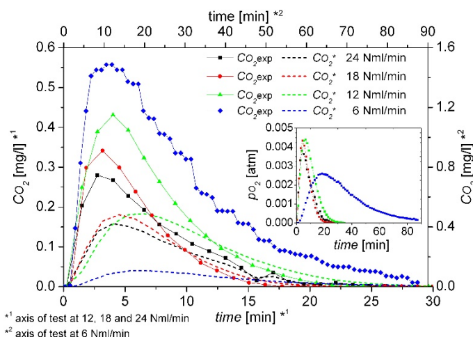
Fig. 3. Experimental data concerning the bubbling experiments performed at different stripping Ar flow rates. C_{O_2exp} and p_{O_2,analyzer} (inset) as function of time (line + symbols) and calculated equilibrium data C_{O_2}^* (dashed lines), at different stripping Ar flow rates.
