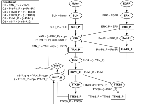
(a) Photoreceptor determination network with miR-7 present.
