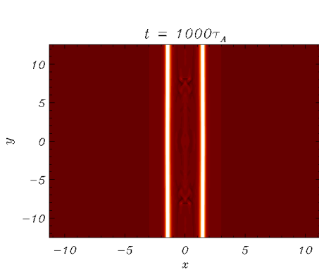
Figure 3. Contour plot of the current density J at t = 1000 in response to the ECCD pulse turned on in the Rutherford regime ( t_1 = 800 ).
