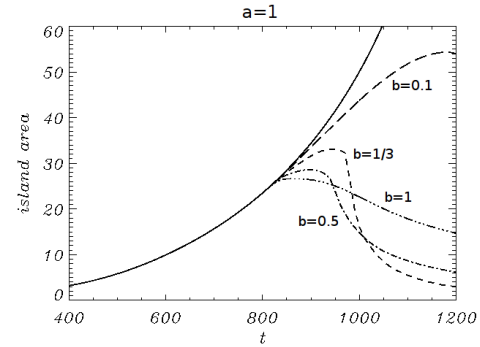
Figure 4. Time evolution of the magnetic island area for control current injections at t_1 = 800 , with various normalized EC beam widths b = \delta/(\psi_X - \psi_O)|_{t_1} and a fixed maximum height J_m = (J_X - J_O)|_{t_1}
