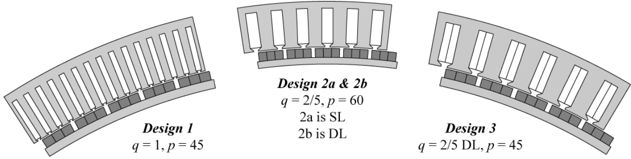
Figure 8. Sketches of the three design examples geometries.
