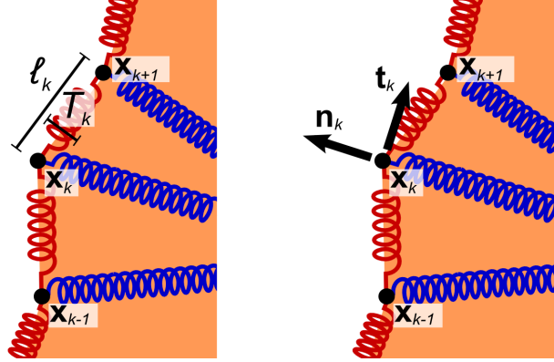
FIGURE 3. Left : A sample discretization of the BM. \mathbf{x}_k and \mathbf{x}_{k+1} identify the k -th rectangle, with length \ell_k and thickness T_k . Right : Normal and tangential vectors for point \mathbf{x}_k ; see Equations 1.
