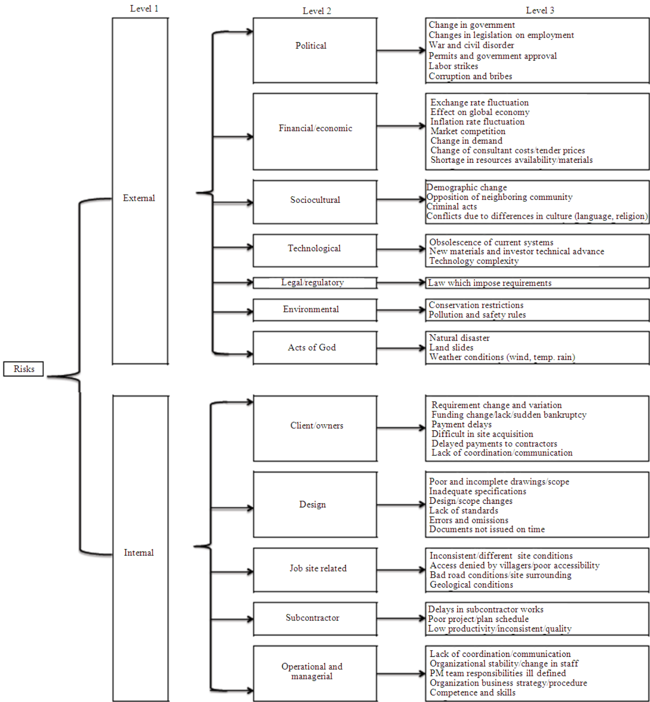
Fig. 1. Proposed taxonomy
