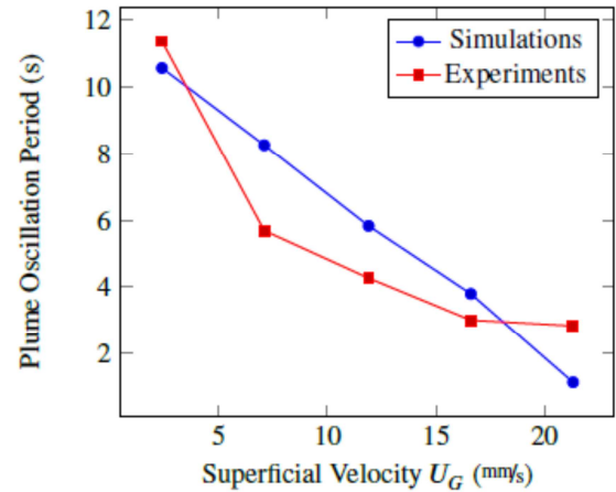
Figure 4: Comparison between experimental data and predicted Plume Oscillation Period for different gas superficial velocities.
