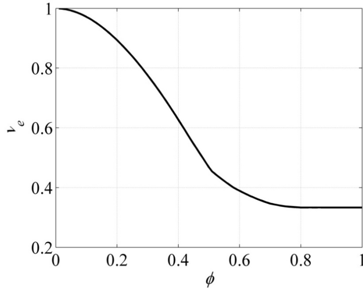
Fig. 3.2 The effective Poisson's ratio \nu_e of the regular hexagonal honeycomb with \nu_s = 1/3 vs the relative density \phi .
