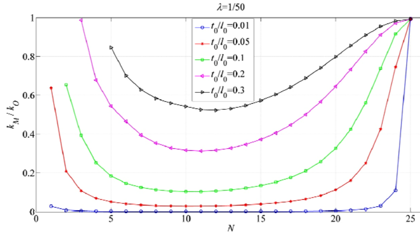
Fig. 3.5 The relative bulk modulus G_M/G_O vs N for different t_0/l_0
