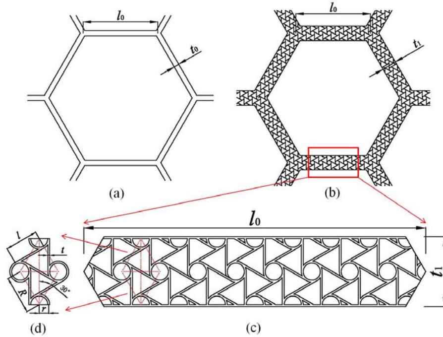
Fig. 4.5 Schematics of (a) the ORHH; (b) the tailorable MHH with chiral honeycomb sub-structures; (c) amplification of a chiral lattice cell wall in (b); (d) geometrical parameters of the chiral honeycomb cell in (c).
