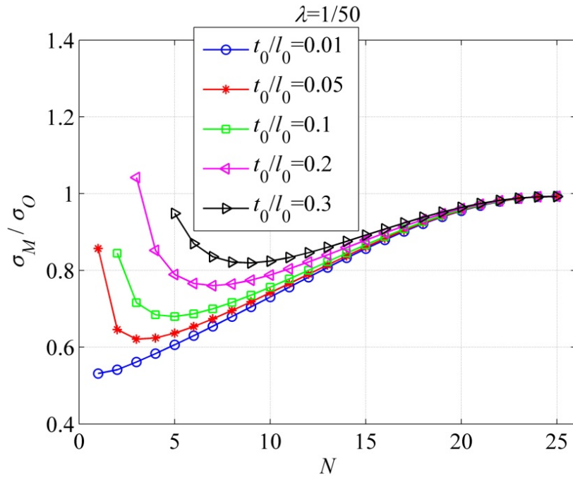
Fig. 3.6 The relative thermal conductivity G_M/G_O vs N for different t_0/l_0
