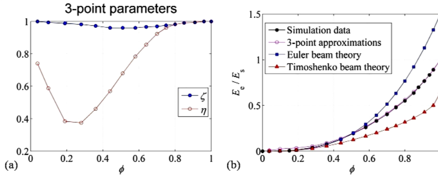
Fig. 3.1 (a) Three-point parameters \zeta and \eta for the regular hexagonal honeycomb ( Hyun and Torquato, 2000 ) vs the relative density \phi ; (b) Effective Young's modulus E_e/E_s of the regular hexagonal honeycomb vs the relative density \phi predicted by different methods.
