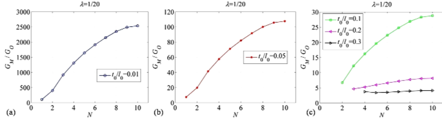
Fig. 3.15 The relative shear modulus G_M/G_O vs N for different t_0/l_0 : (a) t_0/l_0 = 0.01 ; (b) t_0/l_0 = 0.05 ; (c) t_0/l_0 = 0.1, 0.2, 0.3 .
