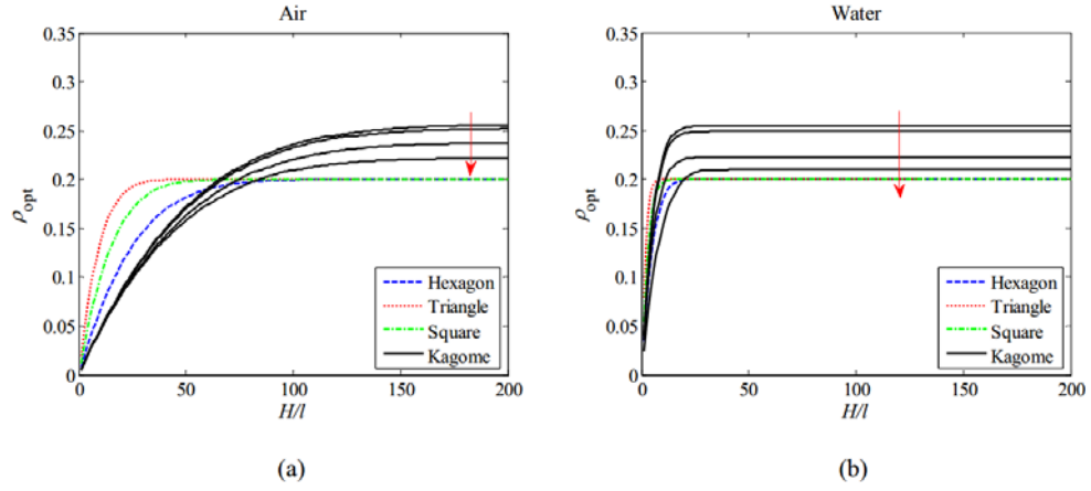
Fig. 2.4 The optimum relative density \rho_{\text{opt}} vs H/l for (a) air; (b) water.
