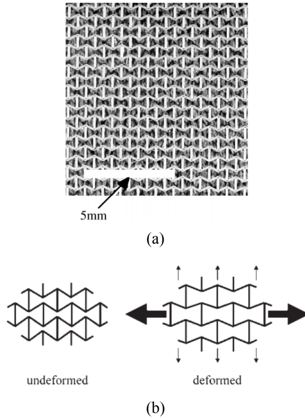
Fig. 1.6 (a) Polymeric re-entrant honeycomb membrane fabricated by femtosecond laser ablation. Pores are approximately 1 mm in width along the horizontal direction ( Evans et al., 2000 ); (b) re-entrant honeycomb in the undeformed and deformed states ( Alderson and Alderson, 2007 ).
