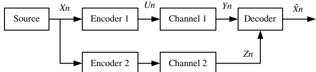
Fig. 2 Compression with transmission of side information.
