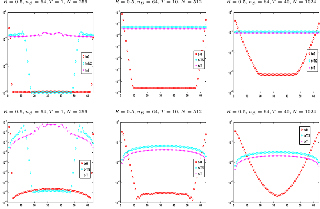
Figure 14: Circular boundary \mathcal{B} : R = 0.5 , n_{\mathcal{B}} = 64 . The first row of the single layer matrices \mathbf{V}_j (top row), and of the double layer matrices \mathbf{K}_j (bottom row).
