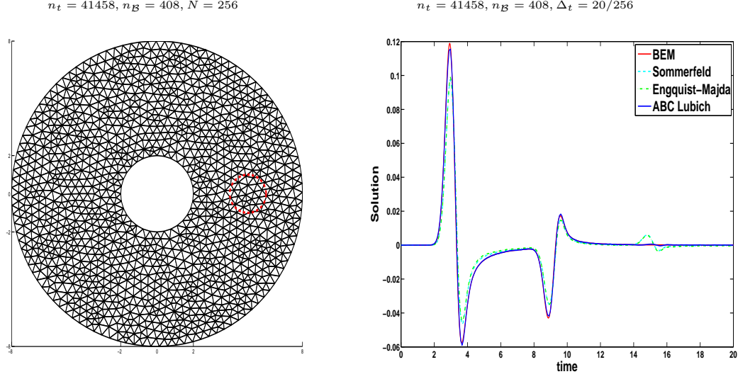
Figure 4: Example 3. Domain triangulation and solution at (8, 0) .
