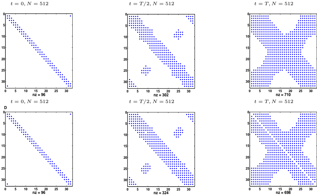
Figure 17: Nut shape boundary \mathcal{B} : n_{\mathcal{B}} = 32 . The single layer matrices \mathbf{V}_j (top), the double layer matrices \mathbf{K}_j (bottom), T = 10 .
