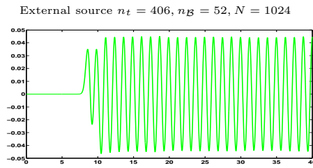
Figure 13: Example 6. The external source case for h(t) = \sin(5t) , \mathbf{x}_0 = (10, 0) .
