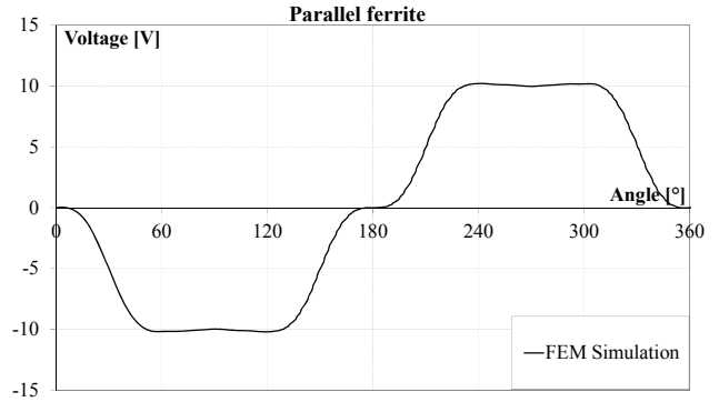
Fig. 7 – Simulated e.m.f. for parallel ferrite motor
