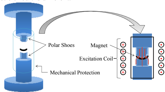
Fig. 2 – Adopted magnetic circuit for the radial magnetization
