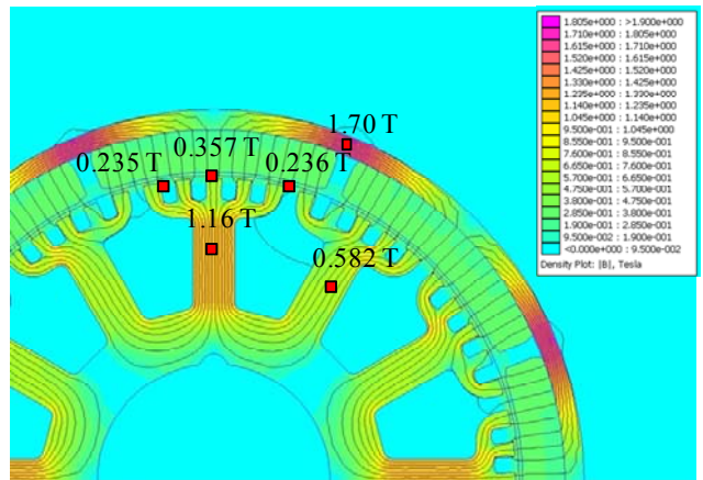
Fig. 9 – Simulated flux density for radial ferrite motor
