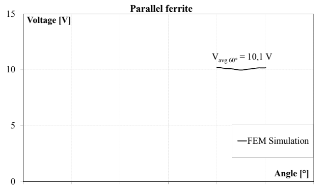
Fig. 8 – Simulated e.m.f. for parallel ferrite motor: waveform and average value V_{dc} during the conduction interval (rectified voltage value)
