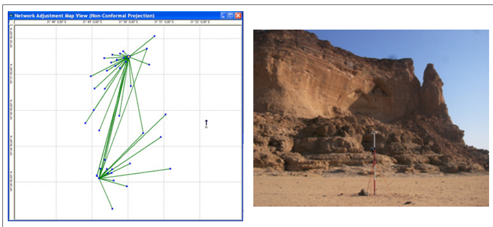
Figure 4 - Final GNSS Adjustment scheme – GNSS Ashtech rover receiver during static session.
