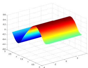
Figure 3: Dirichlet wave problem. Density function \varphi^D .
