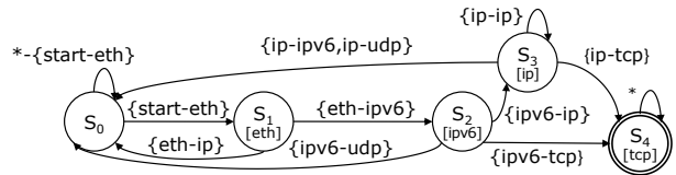
Fig. 7. DFA after the protocol assignment.
