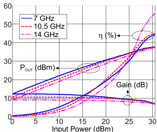
Fig. 8: Simulated output power, efficiency and power gain at 7 GHz (blue solid lines), 10.5 GHz (red dashed lines) and 14 GHz (magenta dot-dashed lines). Bias V_{DS} = 28 V, I_D = 10\% I_{DSS} = 100 mA.
