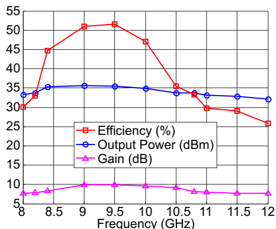
Fig. 10: Single tone amplifier measured behavior in terms of efficiency (red squares), output power (blue circles) and transduced gain (magenta triangles) vs. frequency at compression. Bias V_{DS} = 28 V, I_D = 10\% I_{DSS} = 100 mA.
