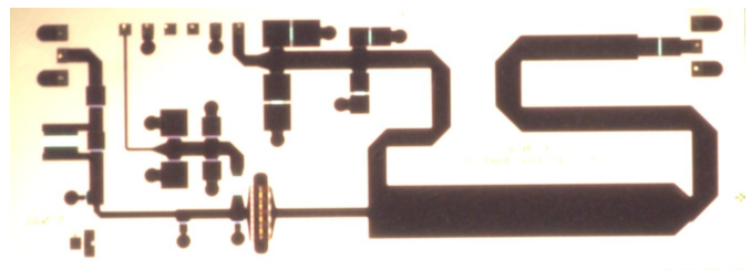
Fig. 6: Microscope picture of the designed MMIC.
