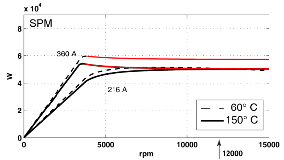
Figure 12. Effect of PM temperature on the power curves of the IPM and SPM motor designs.
