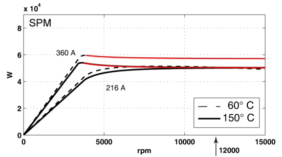
Figure 12. Effect of PM temperature on the power curves of the IPM and SPM motor designs.
