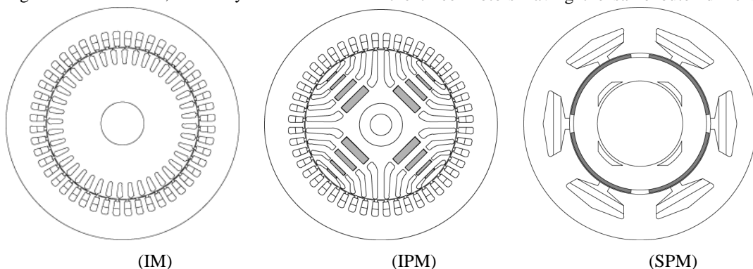
Figure 1. Induction motor, Interior PM motor and Surface mounted PM motor under investigation.
