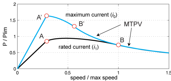
Figure 4. Induction motor power versus speed curves, for rated and overload current amplitudes and limited voltage.
