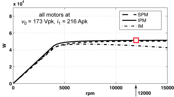
Figure 9. Power curves of the three motors at same current and voltage. SPM and IPM motors fulfill the continuous power specification with the same current and voltage, while the IM requires a higher current.
