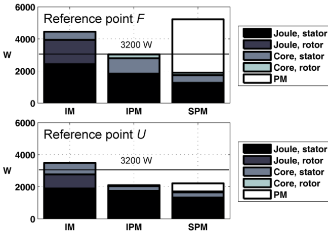
Figure 14. Loss detail in the reference points defined in Fig. 2: a) point F is 39 Nm, 12000 rpm; b) point U is 110 Nm, 4000 rpm.
