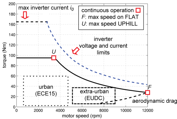
Figure 2. Example of target specification for an electric vehicle.
