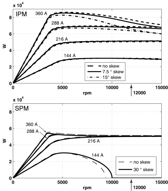
Figure 11. Effect of skewing on the power curves at constant current and voltage of the three design examples.
