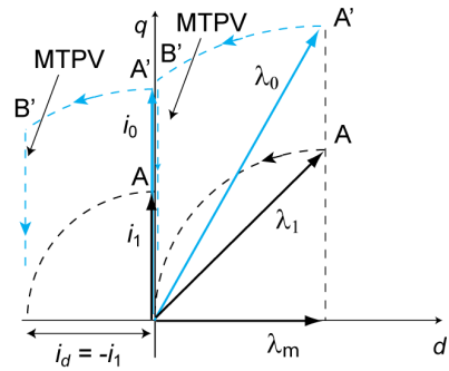
Figure 7. SPM current and flux vector trajectories for maximum power under limited voltage amplitude
