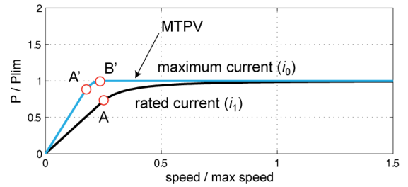
Figure 8. SPM power versus speed curves (limited voltage), for rated and overload current amplitudes
