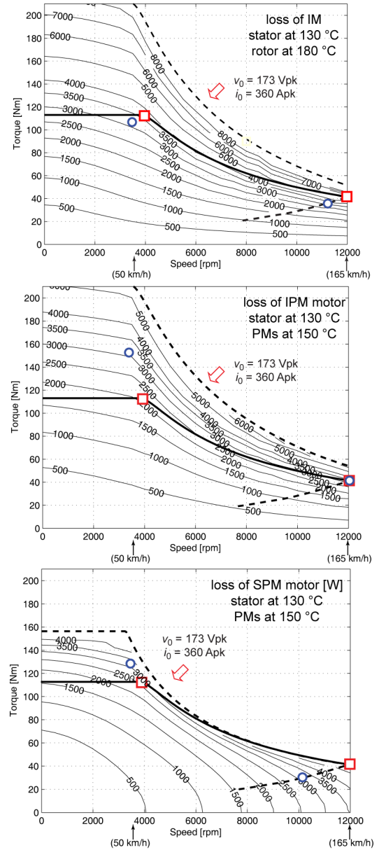
Figure 13. Power loss maps of the three designs over the respective torque versus speed operating regions. The torque limit profiles represent the benchmark continuous operation (continuous line) and the inverter limit (dashed line).
