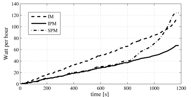
Figure 15. Energy loss over the NEDC driving cycle, for the three motors.
