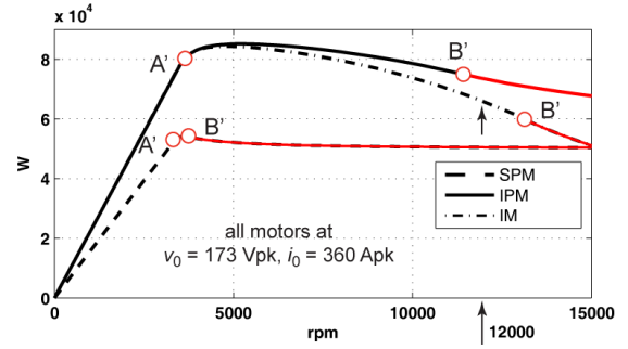
Figure 10. Power curves of the three motors at maximum current and voltage. The continuous red lines, over point B' of the three curves, indicate the MTPV operating region.
