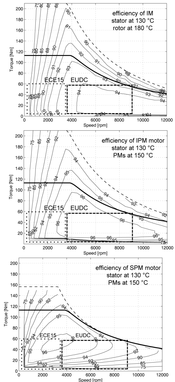
Figure 16. Efficiency maps of the three designs.
