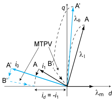
Figure 5. IPM current and flux vector trajectories for maximum power under limited voltage amplitude
