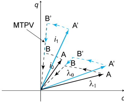
Figure 3. Induction motor current and flux vector trajectories for maximum power under limited voltage amplitude
