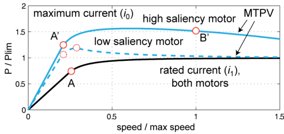
Figure 6. IPM power versus speed curves (limited voltage), for rated and overload current amplitudes. Effect of rotor saliency on the power overload curve:
