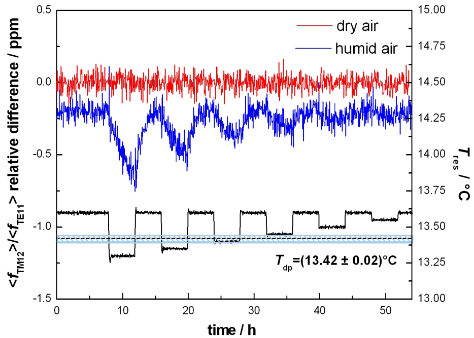
Figure 5.8: Relative difference between the frequency ratio \langle f_{12}^{TM} \rangle / \langle f_{11}^{TE} \rangle measured in humid air (blue line) and in dry air (red line). The resonator temperature profile (black line) is also represented.
