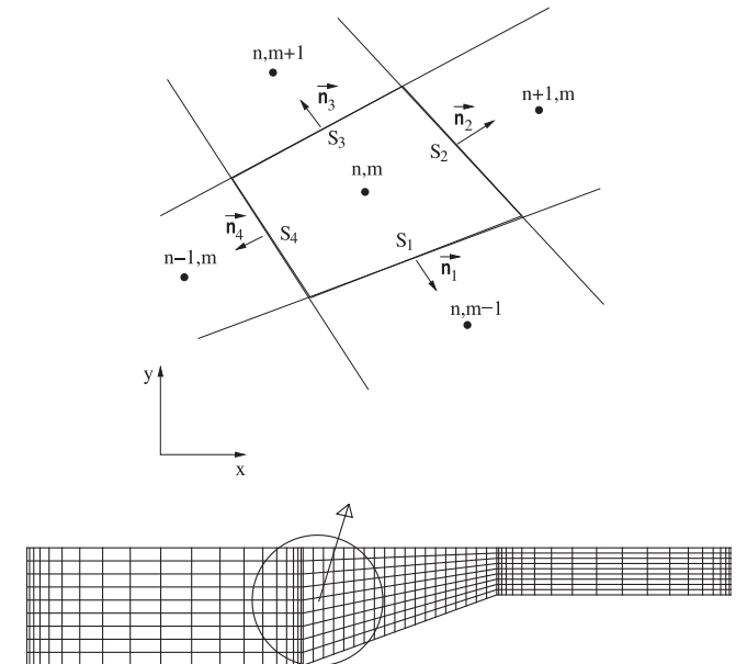
Fig. 1. Two-dimensional computational grid.
