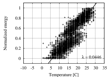
(b) Normalized energy consumption versus external temperature
