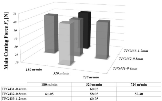
Figure 4. Influence of the cutting speed and tool nose radius on the measured main cutting force, F_z (Depth of cut = 0.5 mm and Feed rate = 0.1 mm/rev).
