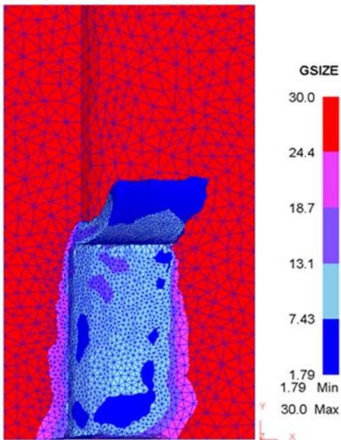
Figure 13. Predicted grain size [ \mu\text{m} ] after calibration of Zener-Hollomon coefficients.
