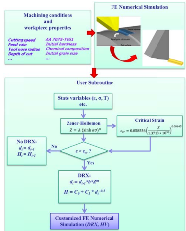
Figure 10. Structure of the user routine for predicting the grain size and hardness.
