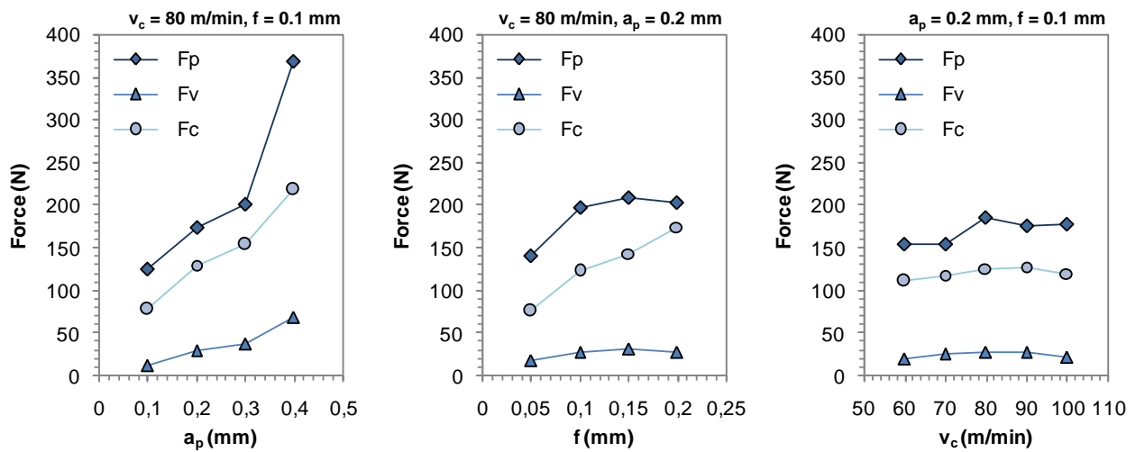
Figure 10: Cutting forces results ( F_c = cutting force, F_v = feed force and F_p = passive force) with RCMX round inserts and for MQL lubrication conditions.
