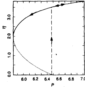
Fig. 18. Example of hysteretic behavior: SP device characteristic corresponding to point A in Fig. 19. The pump power is normalized with respect to P_{th} .
