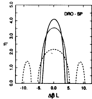
Fig. 14. Curves of conversion efficiency versus phase mismatch in a DRO-SP; the three curves are related to different pump power levels above minimum threshold (—: pump power four times above threshold; .....: ten times; ----: forty times).
