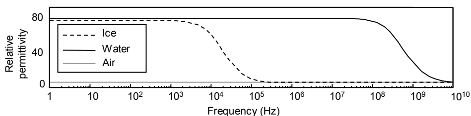
Figure 1. Relative permittivity of water (at 25°C), air, and ice (at -10°C) as a function of frequency.
