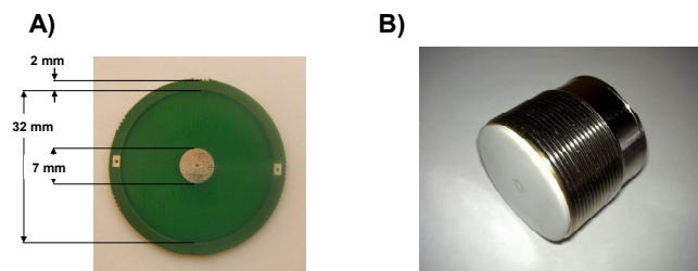
Figure 2. A) The concentric conductive electrodes. B) The sensor.
