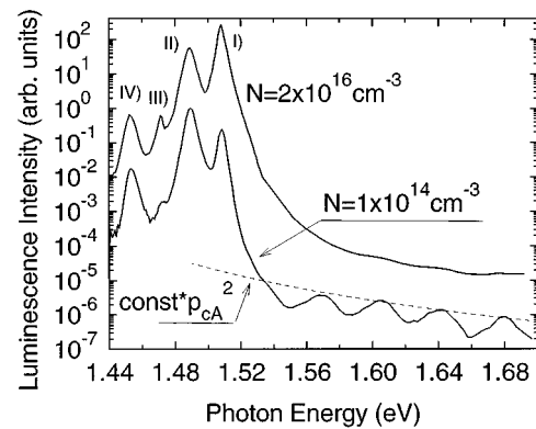
FIG. 1. Total emission spectrum of the p -GaAs sample measured with femtosecond excitation of N=10^{14} and 2 \times 10^{16} electron-hole pairs per \text{cm}^3 . At low photon energies, we observe luminescence peaks due to recombination of thermalized electrons with free holes (I) and with bound holes (II). The peaks at lower energies originate from recombination processes of electrons with free holes (III) and bound holes (IV) involving simultaneous emission of a photon and an optical phonon. The emission at high photon energies is caused by band-to-acceptor recombination of nonequilibrium electrons (peak structure) and by a very weak background due to band-to-band recombination. The dashed line represents the square of the energy-dependent matrix element p_{cA} of the band-to-acceptor transition.
