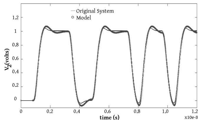
Fig. 9. Output voltage v_2 for the driver and the macromodel (first configuration)
