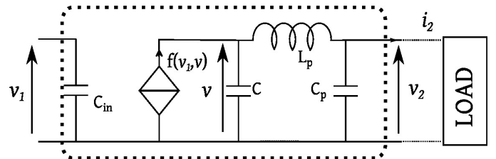
Fig. 1. Synthetic test-system designed to behave like a single-ended driver
