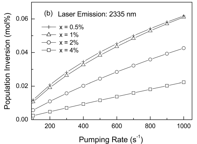
FIG. 9. Calculated population inversion (in mol %) for laser emission at (a) 1865 nm and (b) 2335 nm obtained for Tm 3+(x) -doped TZBG glass with x = 0.5, 1, 2, and 4 \text{ mol \%} . One can find the equivalent pumping intensity ( I_P ) using the relation I_P (\text{kW cm}^{-2}) = 0.02453 \times R_P (\text{s}^{-1}) .
