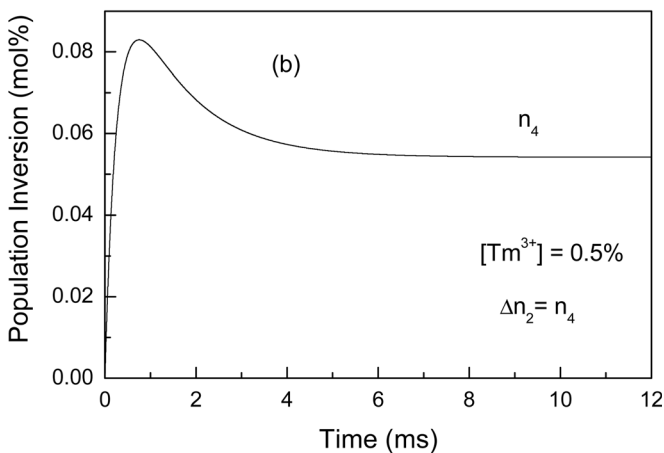
FIG. 8. Calculated evolution of the excited state populations (in mol %) of Tm 3+ for (a) 1865 nm, [Tm 3+ ] = 4 mol % and (b) 2335 nm, [Tm 3+ ] = 0.5 mol % using a pumping rate R_P = 800 \text{ s}^{-1} (or I_P = 19.6 \text{ kW cm}^{-2} ).
