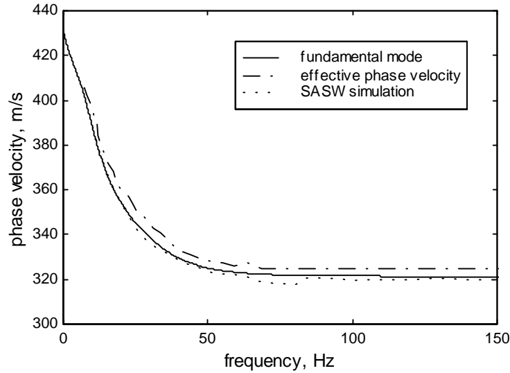
Figure 5.5 Profile A: comparison between dispersion curves
