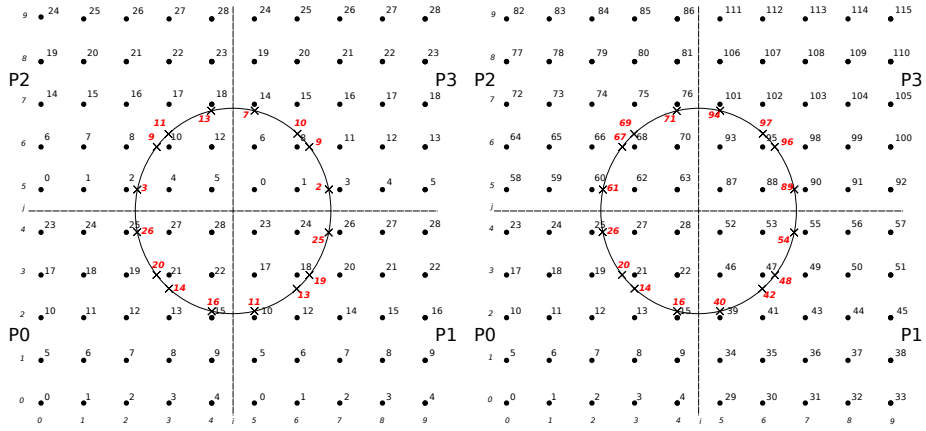
(a) Example of intersections search (4 processors case). The local arrangements; P0, P1, P2, P3. The final global arrangement. Intersections in red. (b) Example of intersections search (4 processors case). The final global arrangement. Intersections in red.
