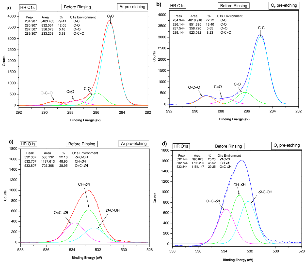
Figure 7.10 XPS spectra of PPAAs deposited after Ar and O 2 etching: a) HR C1s Ar etching; b) HR C1s O 2 etching; c) HR O1s Ar etching; d) HR O1s O 2 etching
