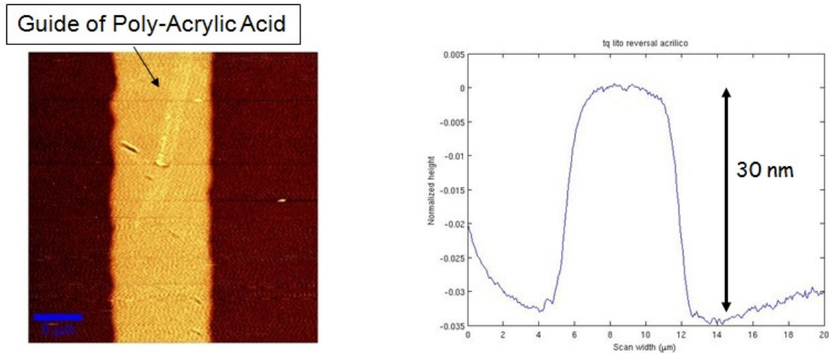
Figure 10.6 PAA strips deposited on the 1DPC surface after lift-off procedure: cross section and profile investigation by AFM
