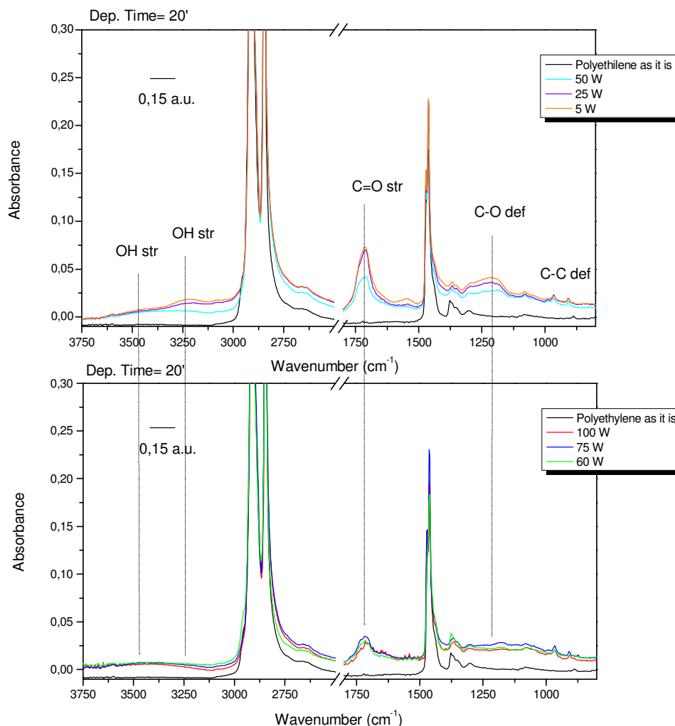
Figure 7.2 FTIR-ATR spectra measured on PE substrates coated with PPAA films obtained in CW plasma processes
