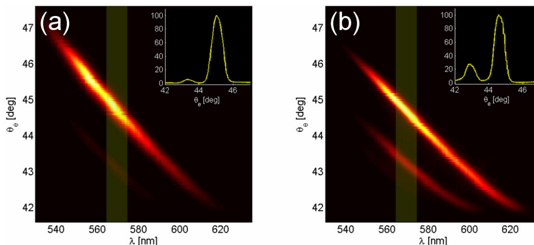
Figure 10.10 Fluorescence maps as measured by a resonant prism-illumination of the high-momentum BSW (localized on ridges). (a) Sample with 5-nm thick PPST layer; (b) sample with no PPST layer. The vertical band indicates the area used for calculating the integrated fluorescence as a function of the detection angle as shown in the inset
