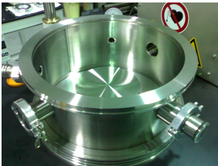
Figure 6.1 The inner of the vacuum chamber of the PECVD reactor
