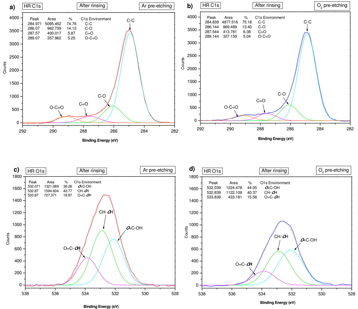
Figure 7.11 XPS spectra collected after rinsing of PAA films deposited after Ar and O 2 etching: a) HR C1s Ar etching; b) HR C1s O 2 etching; c) HR O1s Ar etching; d) HR O1s O 2 etching
