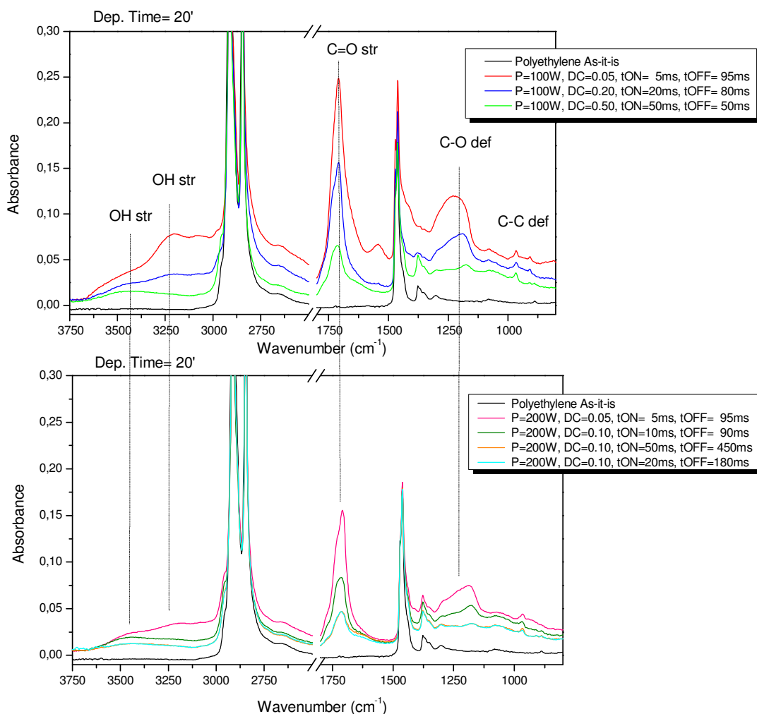
Figure 7.4 FTIR-ATR spectra measured on PE substrates coated with PPAAs obtained in MW plasma processes
