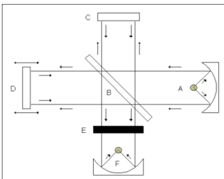
Figure A.5 The schematic of the Michelson interferometer, which forms the basis of most FTIR instruments
