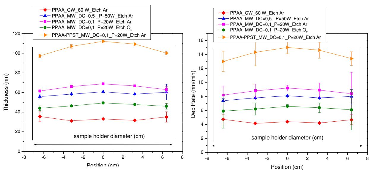
Figure 8.4 Study on the lateral surface homogeneity: the effect of the sample position on the co/polymer deposition rate
