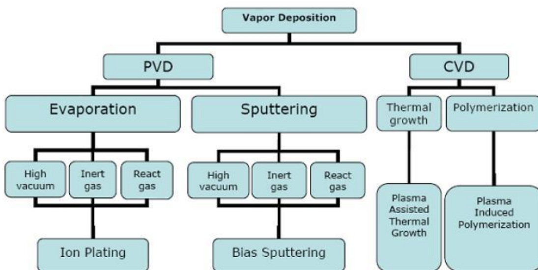
Figure 3.1 Scheme: Vapor Deposition Techniques
