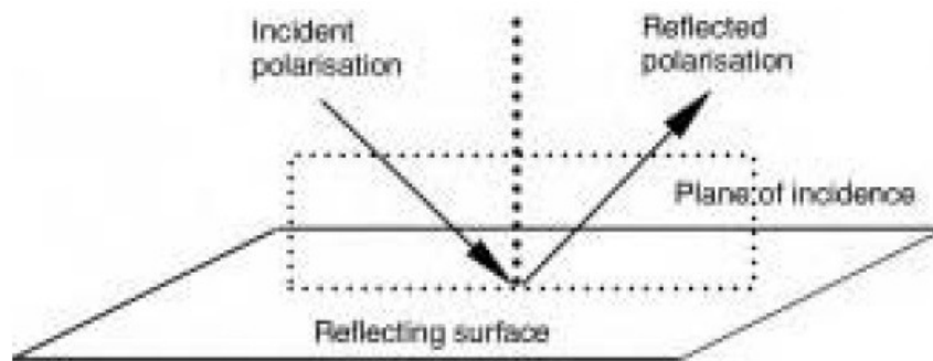
Figure A.7 The geometry of reflection ellipsometry. The change in polarization upon reflection carries information about the characteristics of the sample
