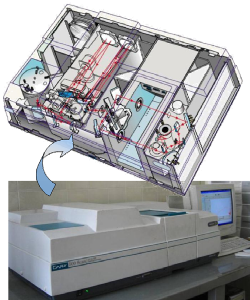
Figure 6.10 CARY 500 Scan UV-Vis-NIR Spectrophotometer and a schematical inner view of the system and the beam path
