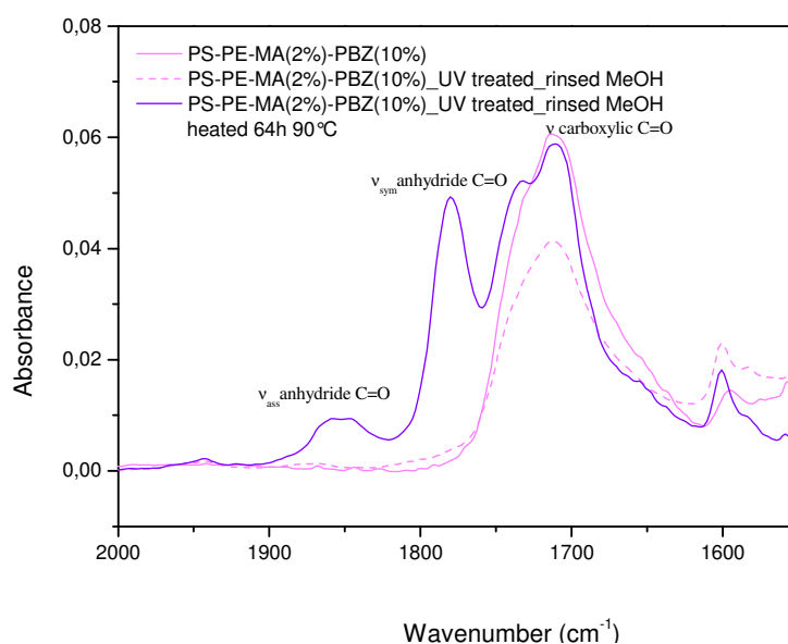
Figure 11. 8 FTIR-ATR spectra of PS functionalized by PEMA (2%) UV immobilized (770 kGy) before (pink solid line) and after rinsing (pink dash line) and after heating treatment for 64 h at 90°C (violet solid line)
