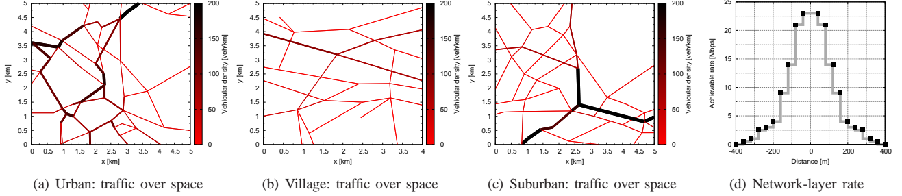
Fig. 4. Road layout in the urban (a), village (b) and suburban (c) scenarios, and achievable network-layer rate characterization as a function of distance (d)
