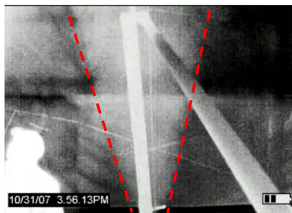
Fig. 7. Frame from the film recorded by the IR camera during a gas release.
