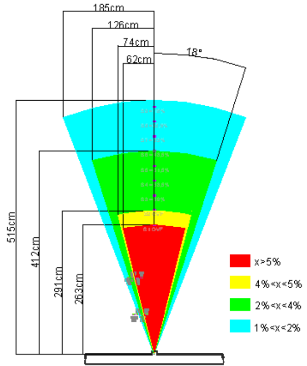
Fig. 10 Gas concentration near the source of release, as determined through experimental data.
