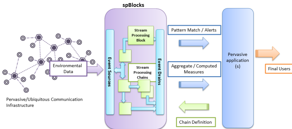
Figure 1: The spChains framework logic architecture.
