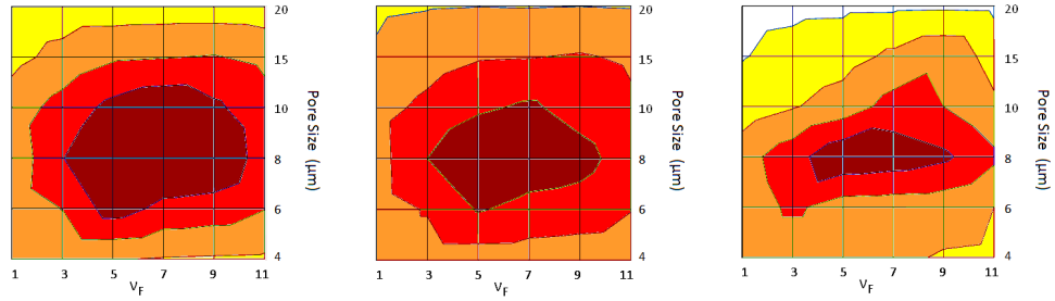
(C) MMP-active cells with rigid nucleus
