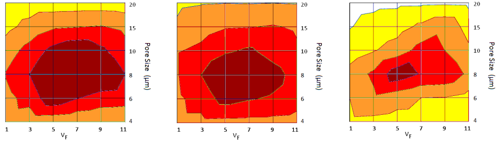
(B) MMP-inactive cells with elastic nucleus
