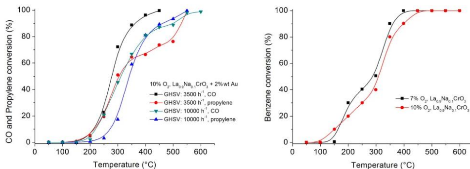
Figure 4. CO, propylene and benzene oxidation tests with supported catalysts.
