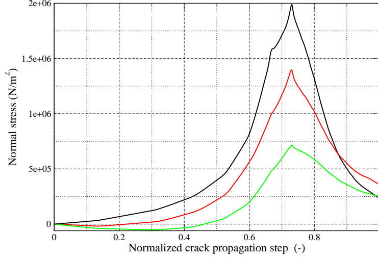
Figure 11: Normal stress at a fixed location ( x = 0 , y = 0.022 m, z = 0.02 m) for notch depth 7.3 mm; upper curve \sigma_x , curve in the middle \sigma_y , lower curve \sigma_z
