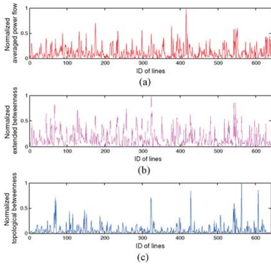
Fig. 1. Criticality of lines measured by various scenarios in Italian power grid. (a) Criticality of lines through normalized averaged power flow. (b) Criticality of lines through normalized extended betweenness. (c) Criticality of lines through normalized topological betweenness.
