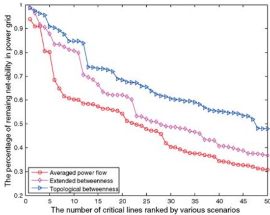
Fig. 3. Remaining net-ability in the Italian power grid after removing 50 most critical lines in various scenarios.
