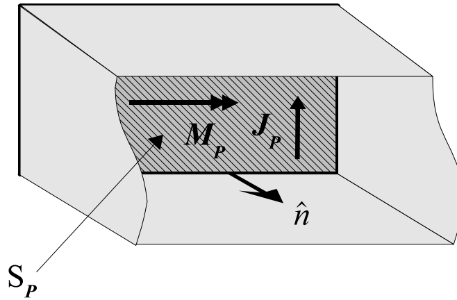
Figure 2. Electric and magnetic equivalent current densities are defined over the waveguide port aperture.
