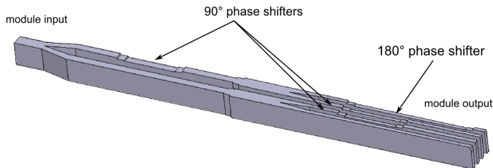
Figure 8. RF model of the 4-active and 4-passive multi-junction.
