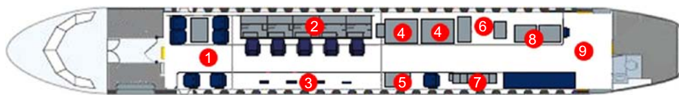
Figure 5 Systems and crew accommodation
