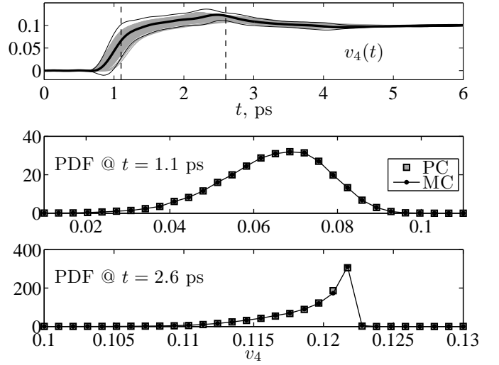
Fig. 10. Transient response v_4(t) for the nanointerconnect of this study (top panel) and its PDF (bottom panel). The curves in this figure are computed with \mathcal{L} = 20 \mu\text{m} , \tau = 0.3 ps and C_L = 10^{-4} pF. The same notation of Fig. 9 applies here.
