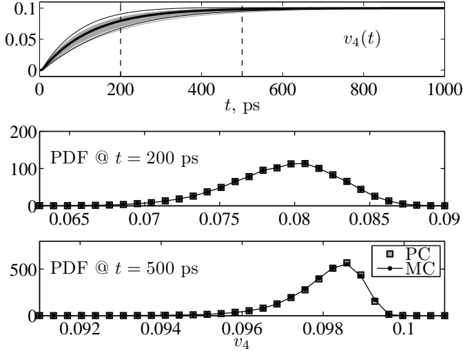
Fig. 9. Top panel: transient response v_4(t) for the nanointerconnect of this study, with \mathcal{L} = 100 \mu\text{m} , \tau = 3 ps and C_L = 10^{-2} pF. Solid black thick line: deterministic response; solid black thin lines: 3\text{-}\sigma limits of the third-order PC expansion; gray lines: a sample of responses obtained by means of the MC method (limited to 100 curves, for graph readability). Bottom panels: probability density function of the near-end crosstalk v_4(t) computed at different times. Of the two distributions, the one marked MC refers to 40,000 MC simulations, while the one marked PC refers to the response obtained via the PC expansion
