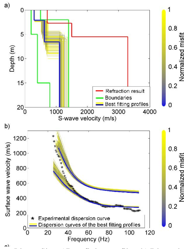
Figure 4 Varese Figure Site: a) Best fitting profiles; b) Dispersion curves of soil profiles compared with the experimental dispersion curve.
