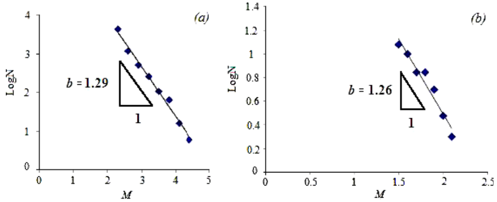
Figure 3. GR distribution of magnitudes for AE events in the pillar (a) and nearby seismicity (b). The magnitude of AE events is defined by the relation M = \log(V/1 \mu\text{V}) where V is the peak amplitude (expressed in volt) of AE signals, while M means the Richter magnitude for earthquakes.
