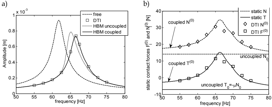
Fig. 16. (a) Comparison of the forced responses of the left blade calculated by means of different strategies (DTI vs. HBM) and (b) corresponding static contact forces on the damper
