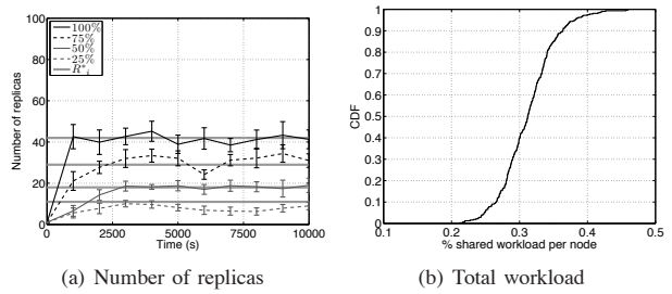
Fig. 3. Impact of content popularity on the replication with shared capacity, in terms of number replicas, workload distribution
