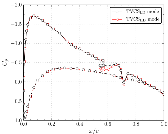
Fig. 6 Pressure coefficient distributions on the LD (◁) and HD (○) modes. \alpha = 6^\circ .
